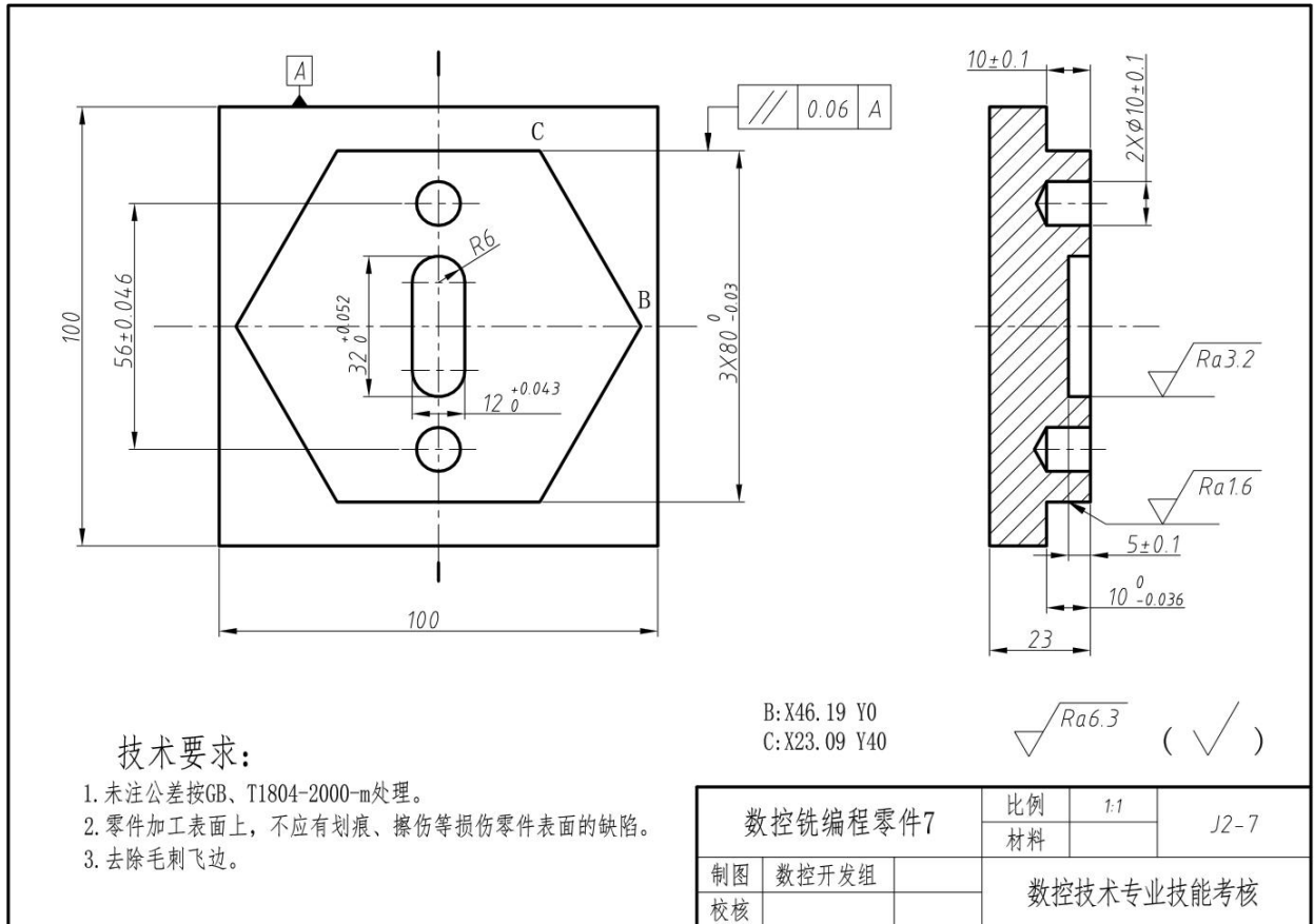
图J2-7 数控铣编程零件7
