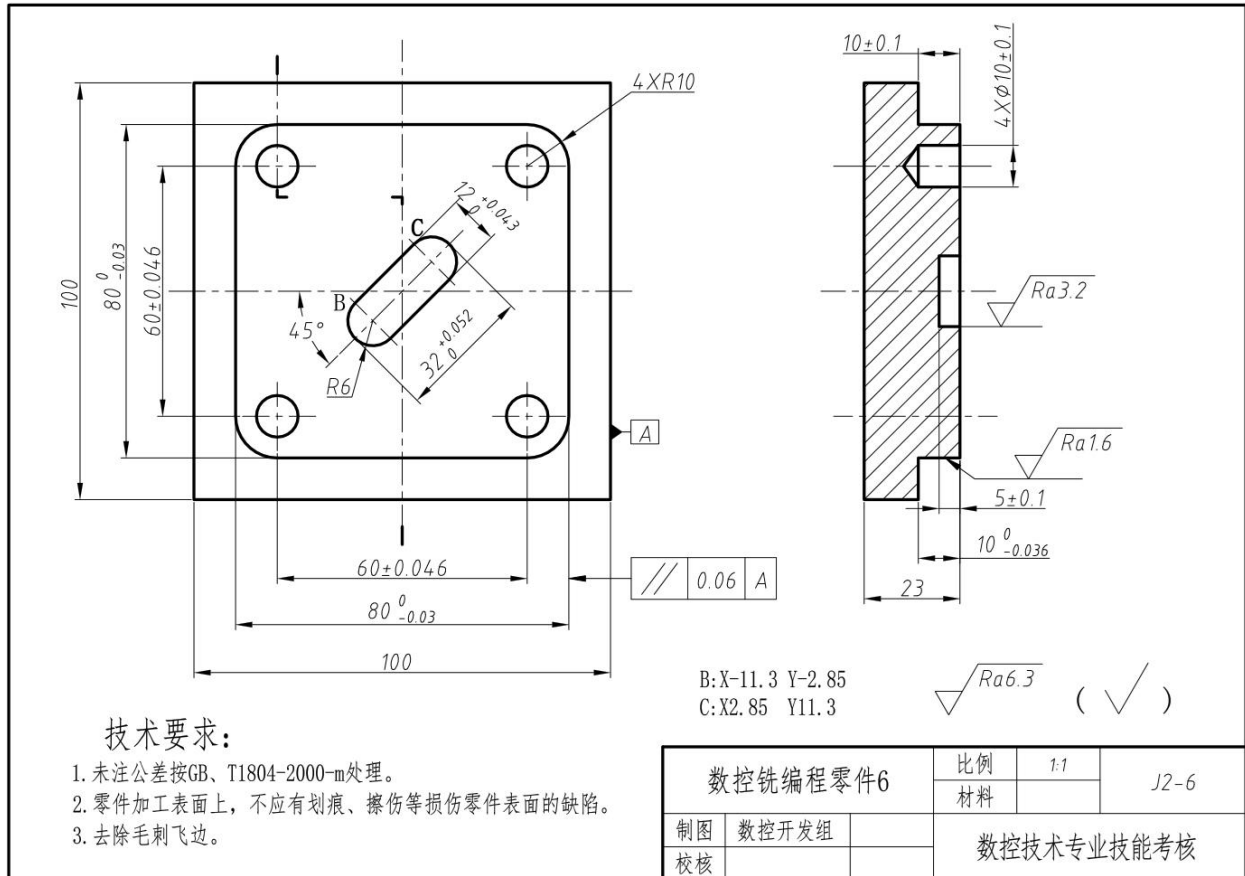
图J2-6 数控铣编程零件6
