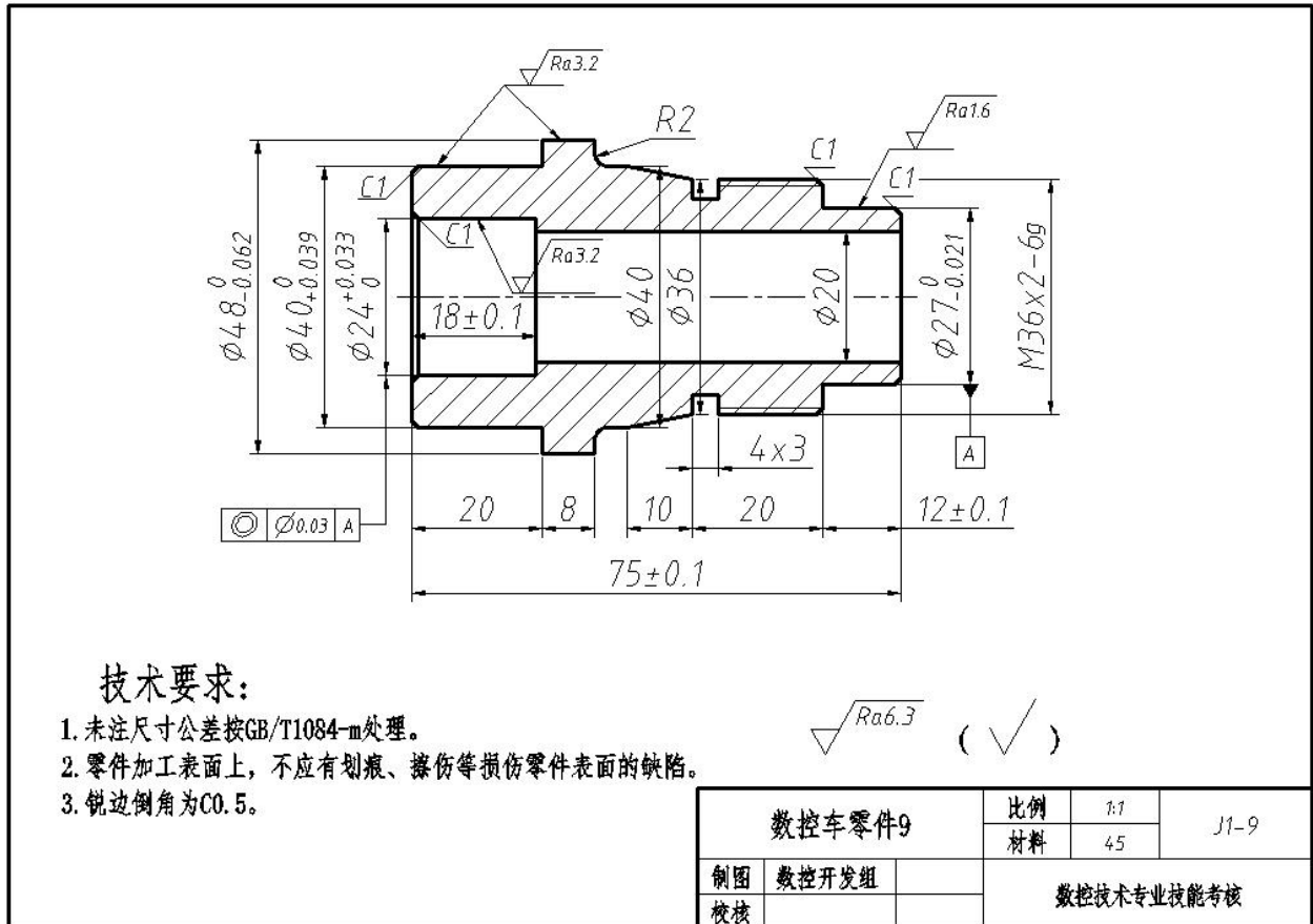
图J1-9 数控车零件9
