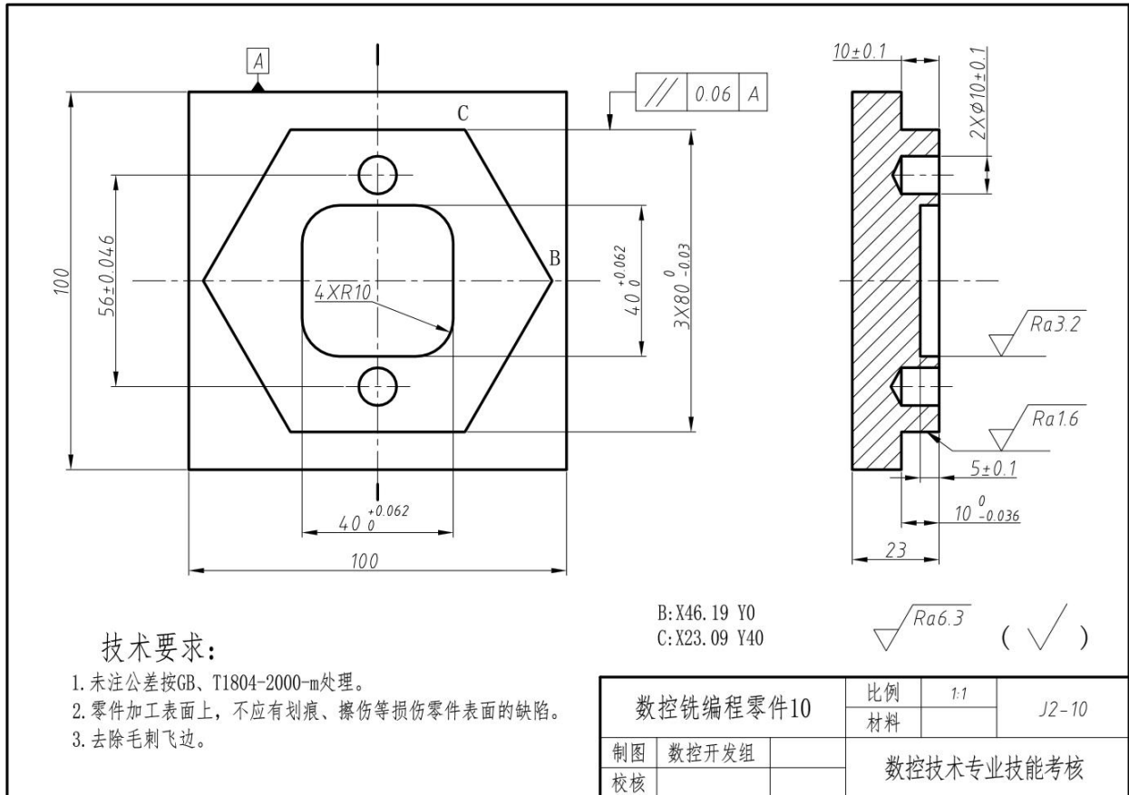
图J2-10 数控铣编程零件10
